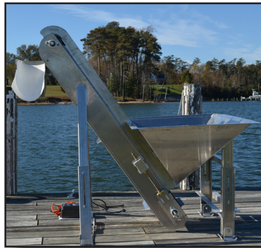
One-Piece Elevator Conveyor
